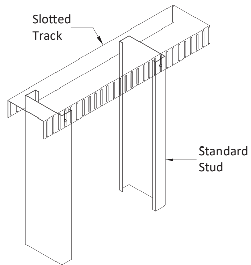
Slotted Deflection Track
